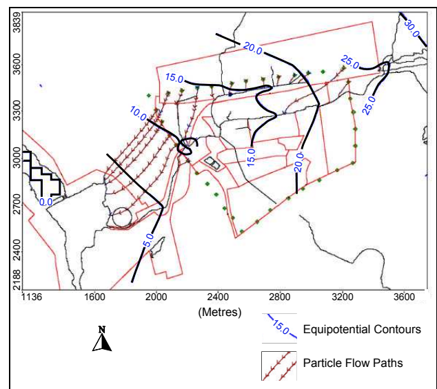
Figure 10. Steady State Particle Tracking, Moderate Flow Conditions, Fill Layer
