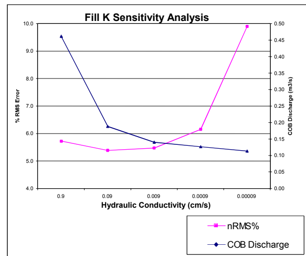
Figure 11. Sensitivity Analysis Example - Fill Conductivity
