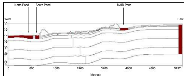
Figure 8. Cross-section of Specified Head Boundary conditions
