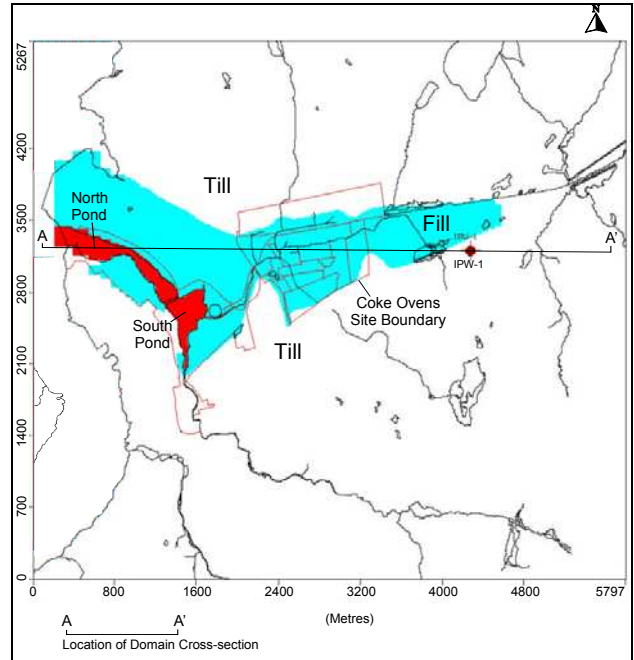
Figure 4. Plan view distribution of the Fill and Till units
