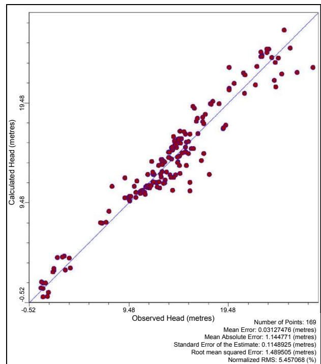
Figure 9. Calculated versus Observed Hydraulic Heads
