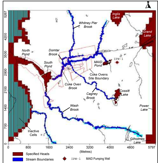
Figure 7. Plan view of Specified Head Boundary conditions
