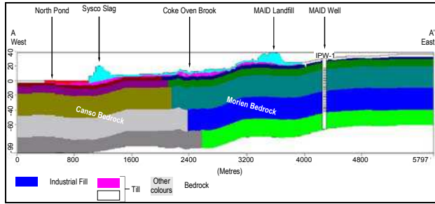
Figure 3. Domain cross-section (see Figure 4 for location)
